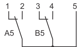
2x change over contacts
