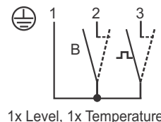
1x Level, 1x Temperature switch
