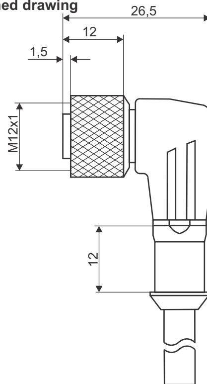
Dimensioned drawing
